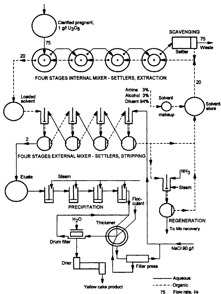
FIG. 5.2. Amine extraction circuit, Kerr-McGee Corp., Grants Mill, New Mexico. Each S-X battery consists of 4 mixer-settlers. Solid lines aqueous, dashed lines organic flow. Numbers are flow rates (l/s).
