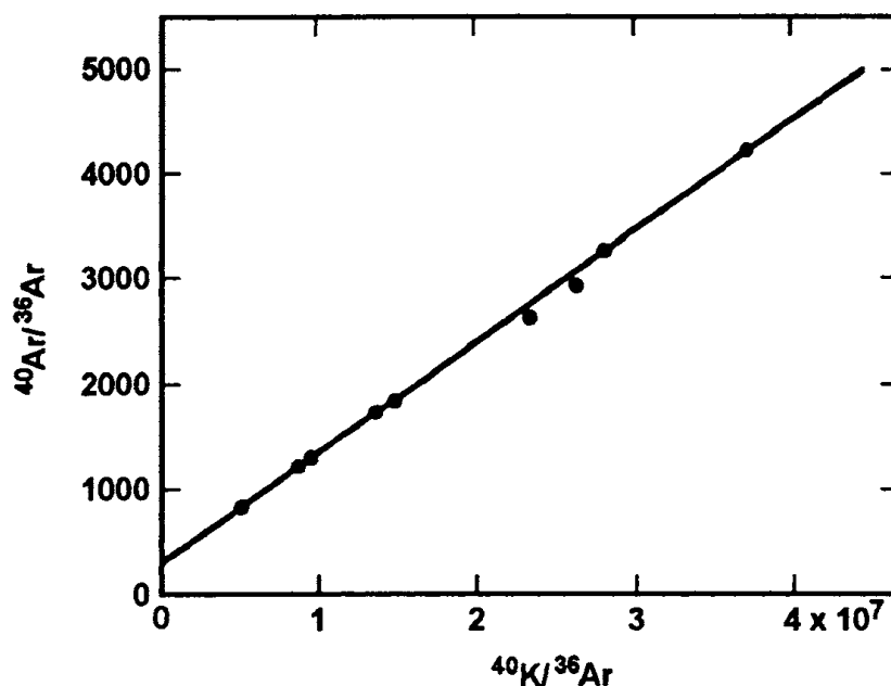
FIG. 5.6. K–Ar isochron of tuff from Olduvai Gorge, Tanzania, yielding a slope corresponding to an age of 2.04 \pm 0.02 My. (From Faure.)
