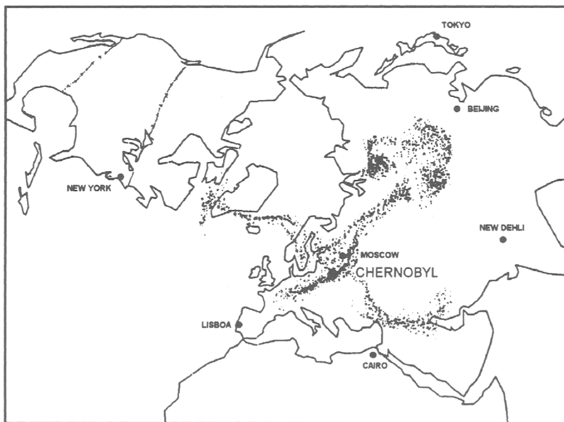
FIG. 5.8. The distribution of the airborne radioactivity from Chernobyl.
