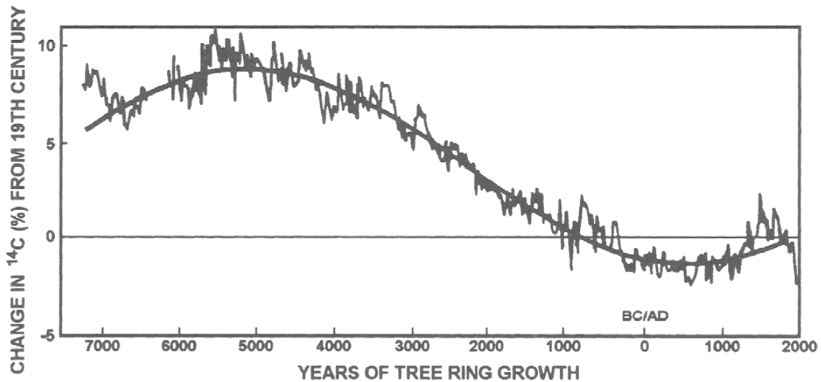
FIG. 5.5. Long term variation in atmospheric ^{14}\text{C} activity as determined from tree rings. (From H. E. Suess, La Jolla Radiocarbon Lab.)
