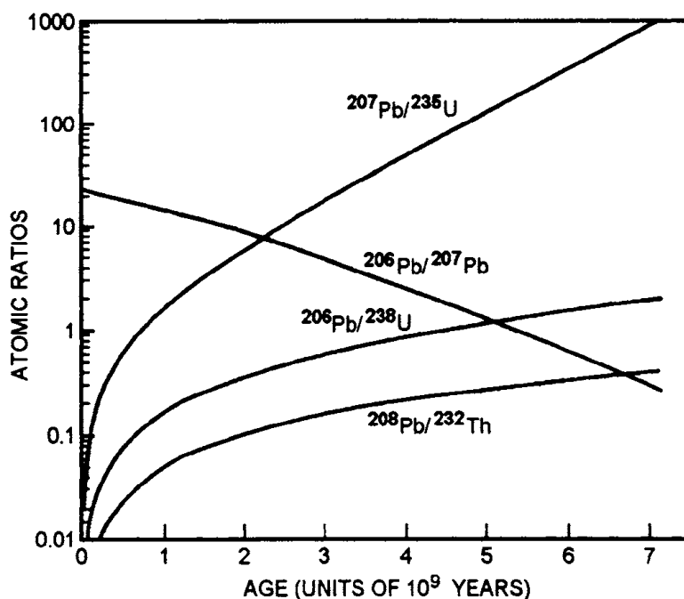
FIG. 5.7. Atomic ratios at the time of measurement as a function of the age of the minerals. (From E. K. Hyde.)
