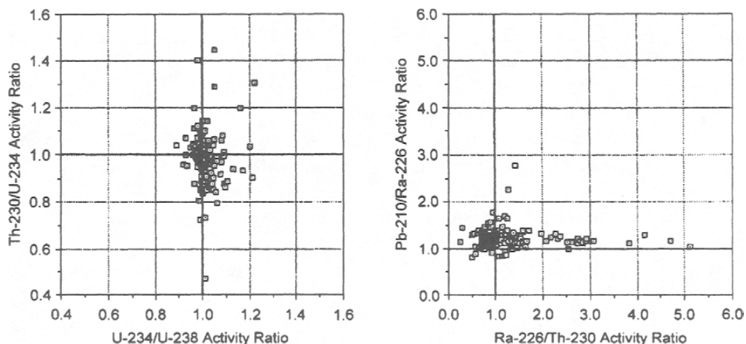
FIG. 5.3. Activity ratios ^{234}\text{U}/^{238}\text{U} vs ^{230}\text{Th}/^{234}\text{U} , and ^{226}\text{Ra}/^{230}\text{Th} vs ^{210}\text{Pb}/^{226}\text{Ra} for rock samples from the Tono uranium deposit. (From Nohara et al.)
