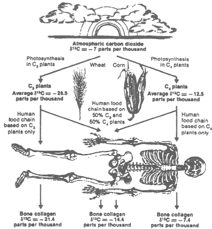
FIG. 5.4. Ratio of ^{13}\text{C}/^{12}\text{C} in human bone depends on diet and affects the \delta^{13}\text{C} correction factor. (From American Scientist, 70 (1982) 602.)
